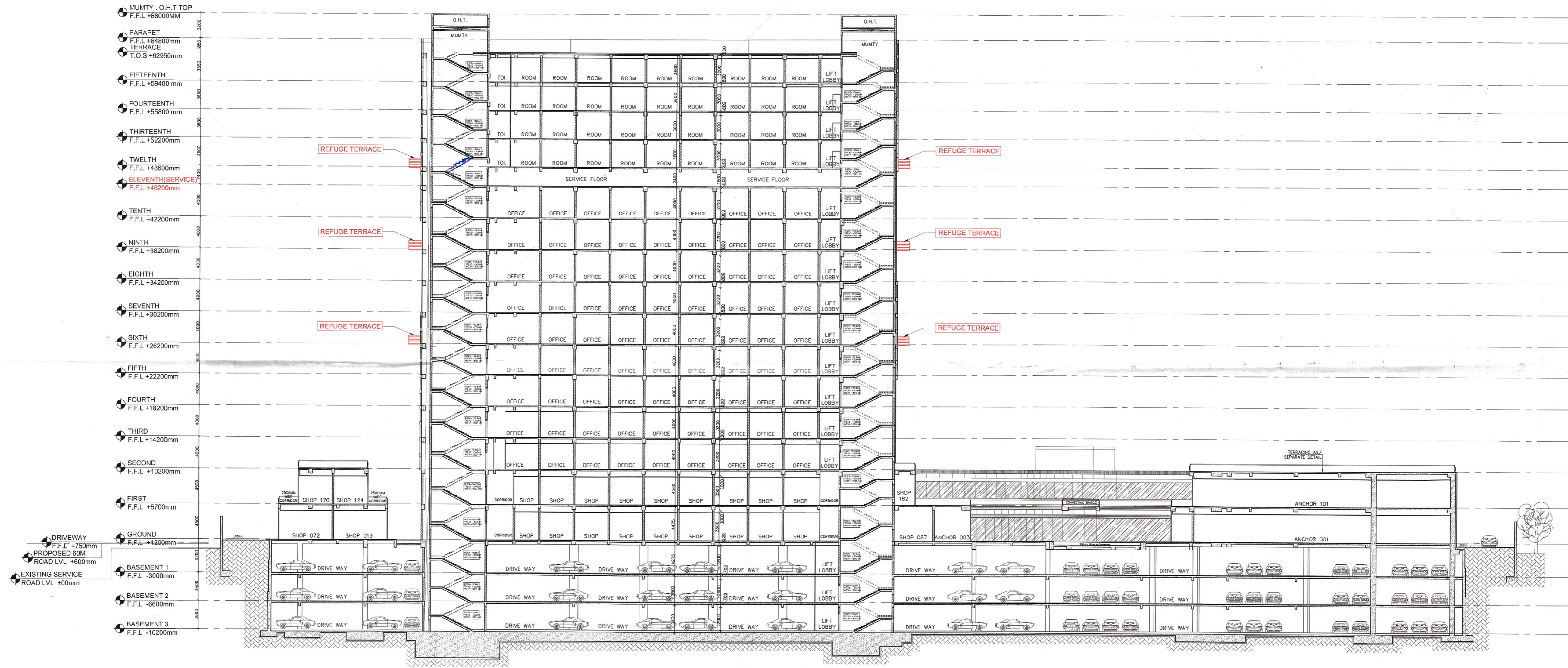
SECTION 1-1
