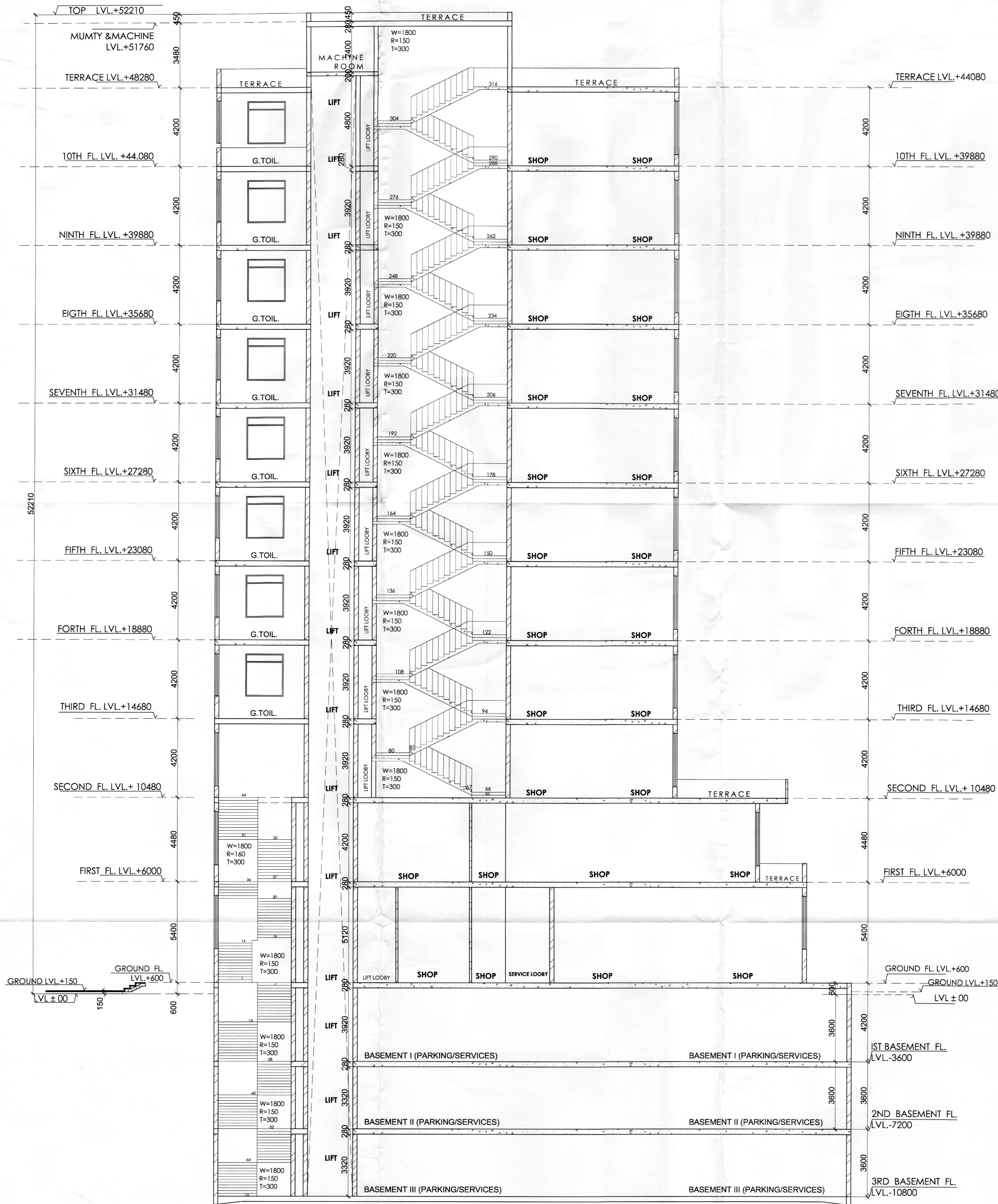
SECTION C-C
